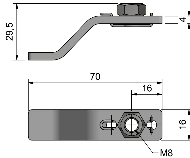
Angled cam 421907, sold separately
